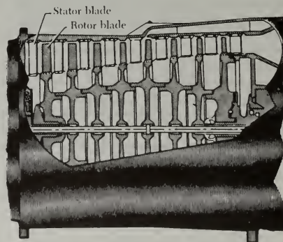
FIGURE 1-42. Disk-type compressor rotor.
